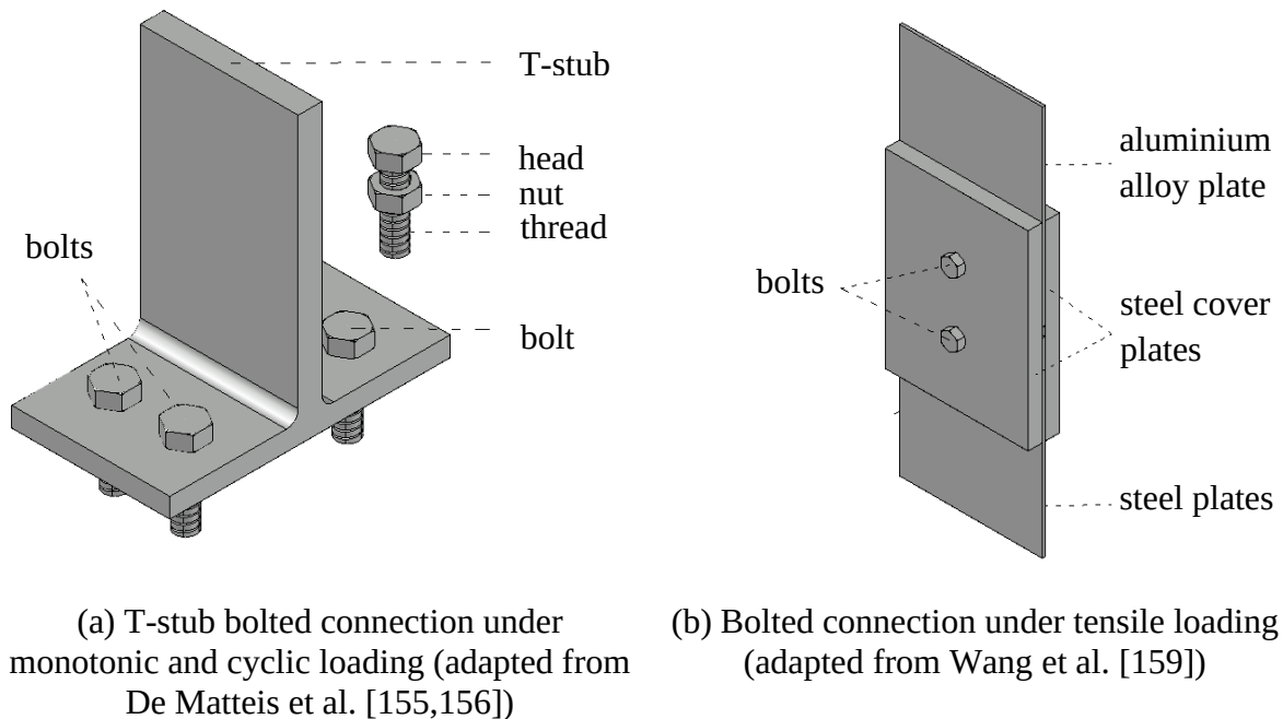
Figure 8: Configuration of investigated bolted connections.
